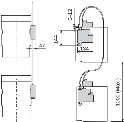
Vertical mounting
