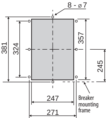
Door frame panel-cut
