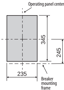
Panel-cut
