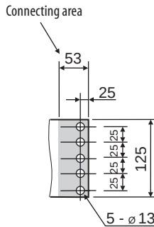
Main circuit terminals
