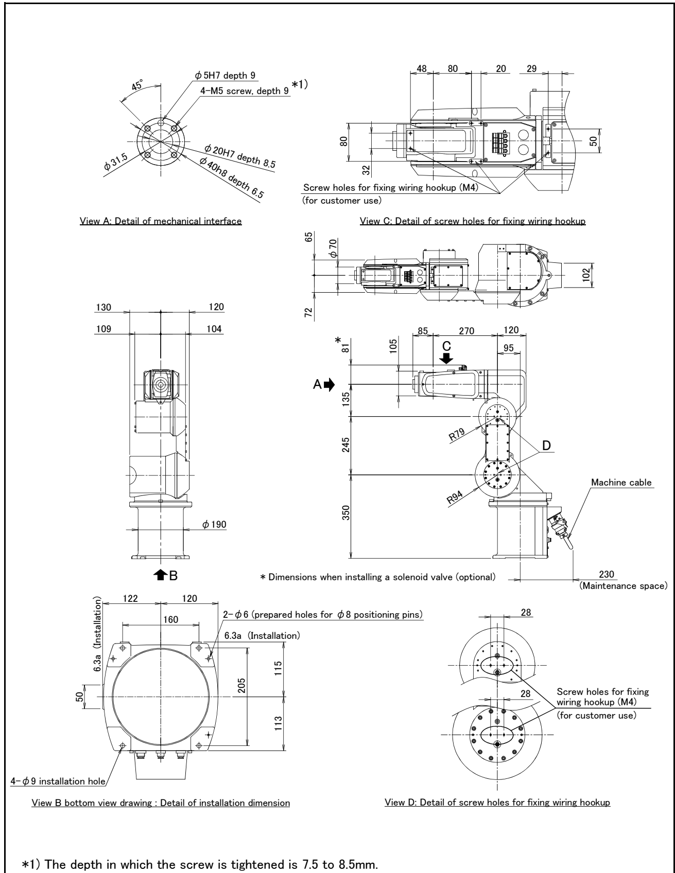
Fig.2-3 : Outside dimensions: (6-axis type)
