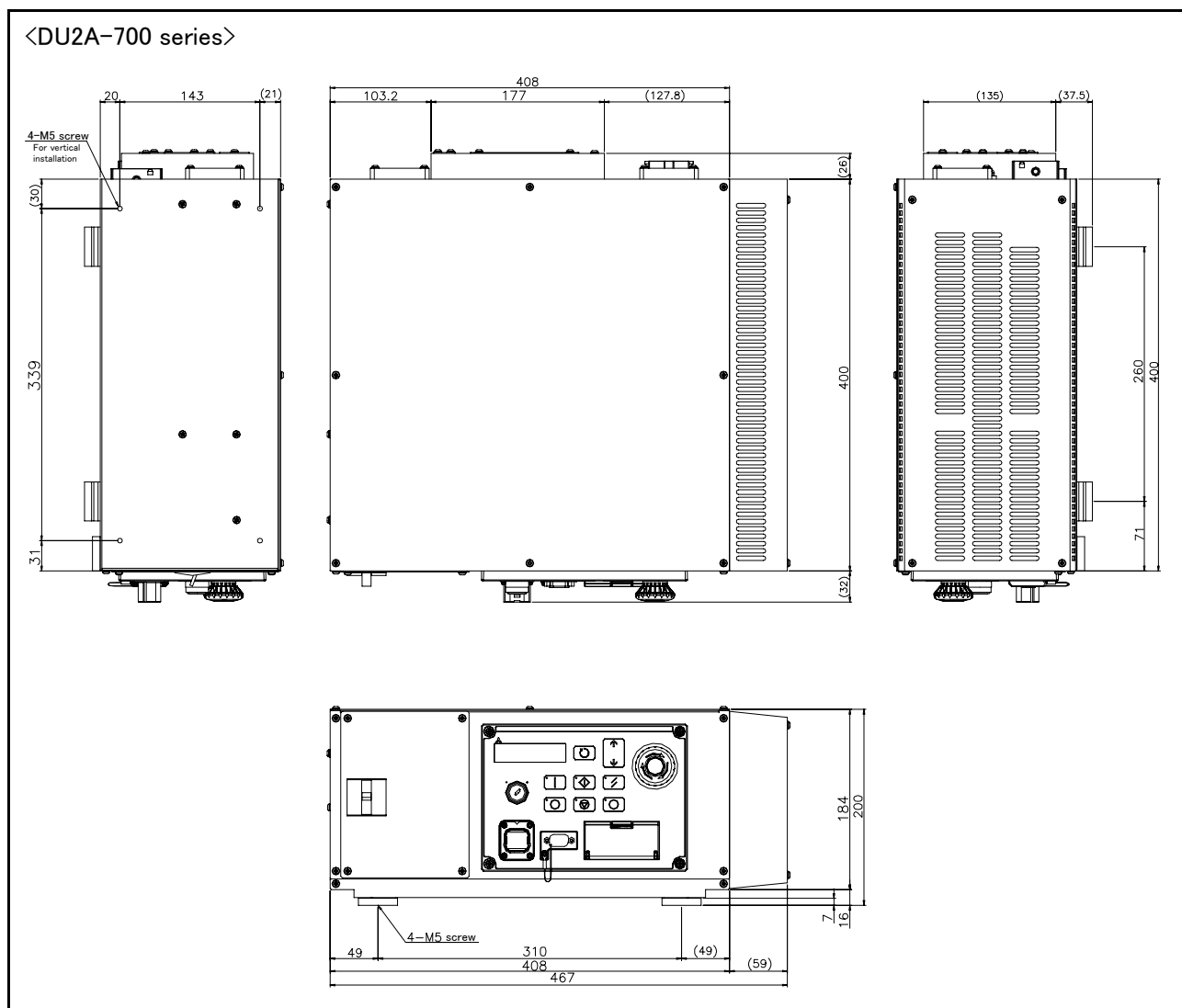
Fig.3-9 : Outside dimensions(DU2A-700 series)
