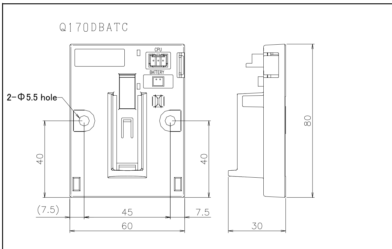
Fig.3-11 : Outside dimensions of battery unit
