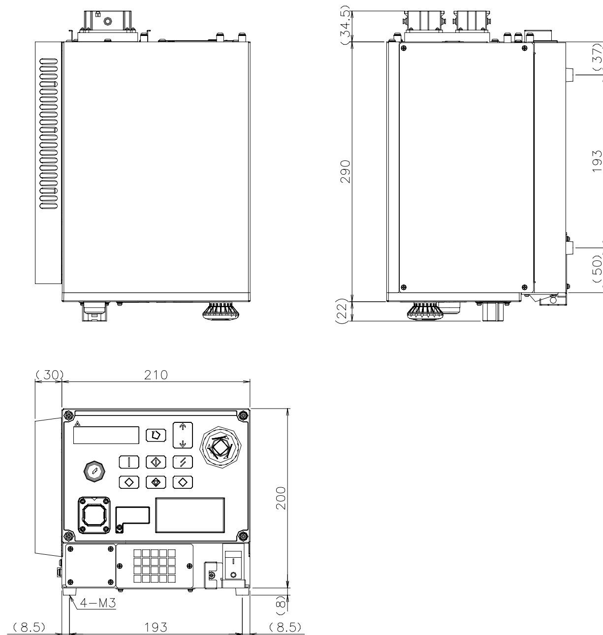
Fig.3-7 : Outside dimensions(DU1A-700 series)
