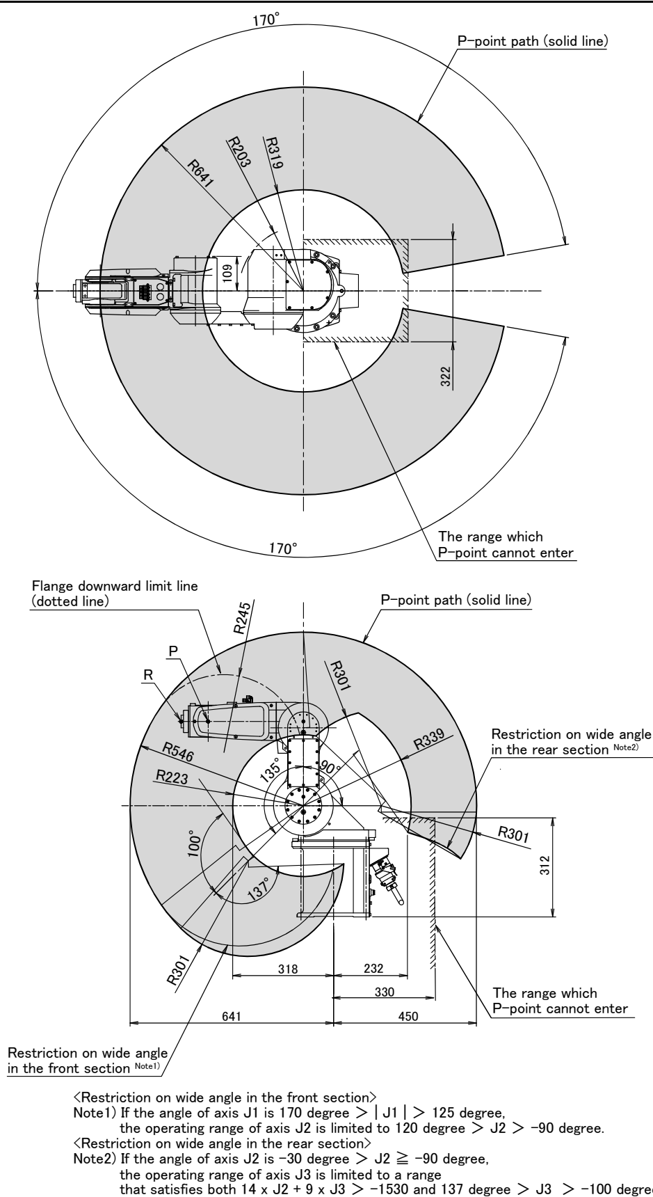
Fig.2-6 : Operating range diagram: (5-axis type)
