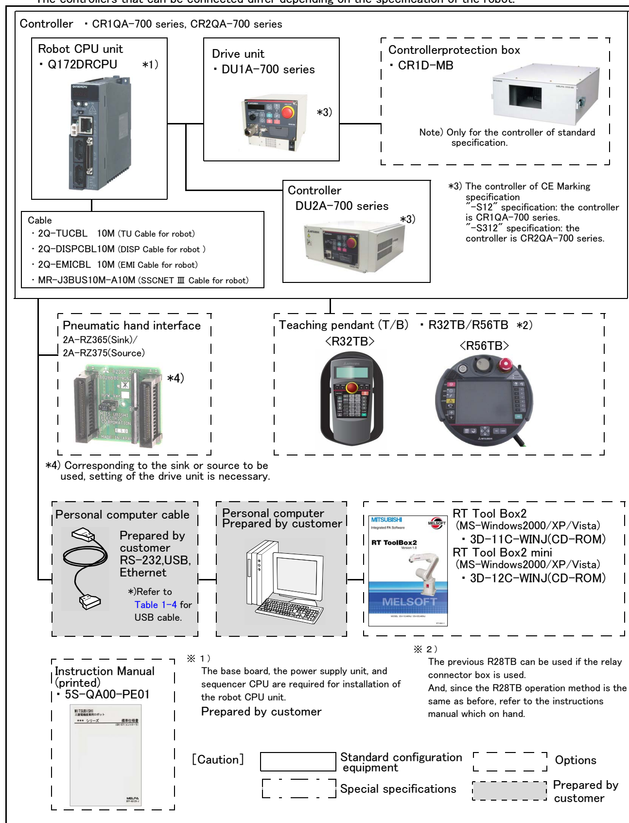
Fig.1-2 : Structural equipment
