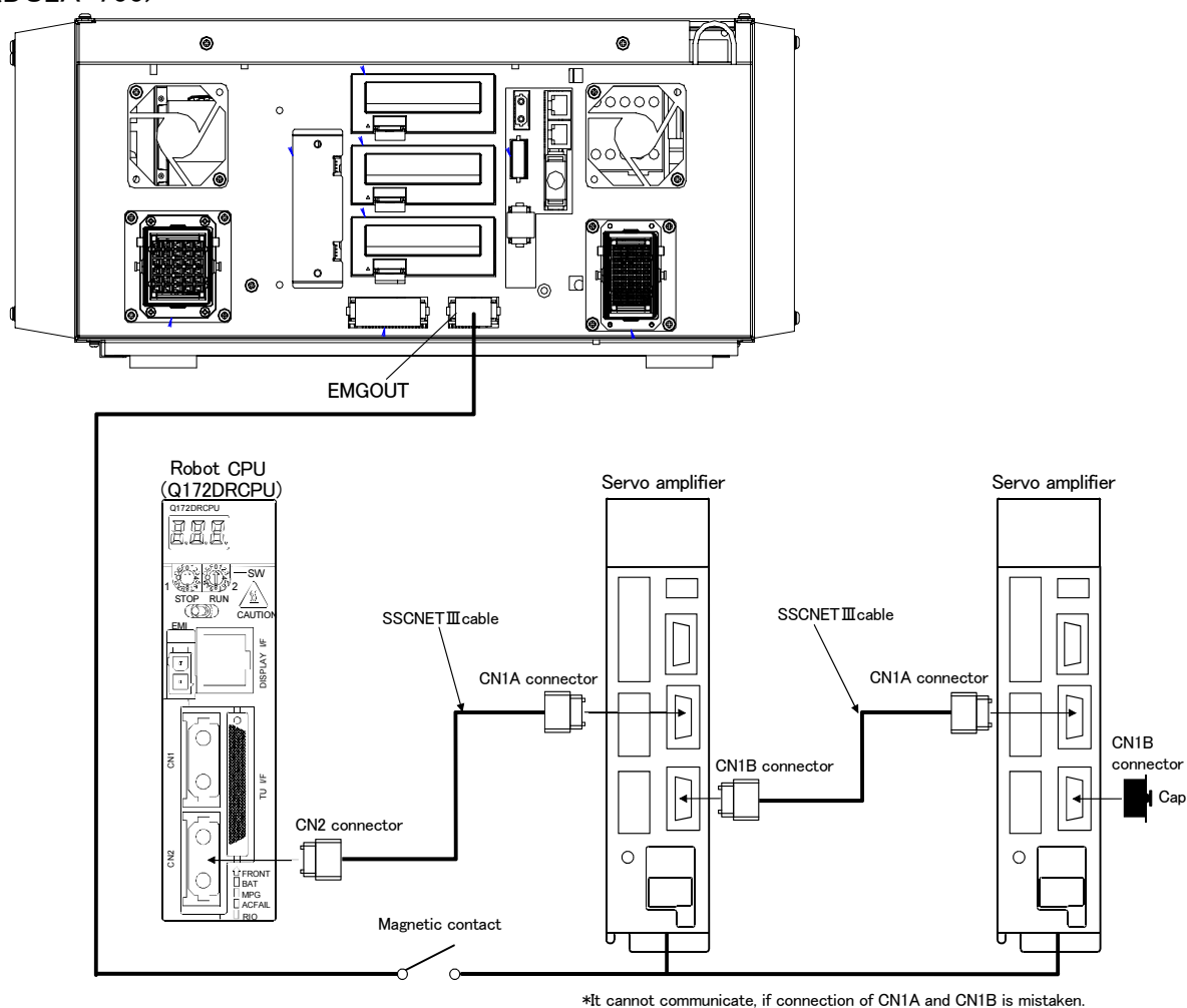
Fig.3-25 : Example of addition axis connection (DUA2-700)
