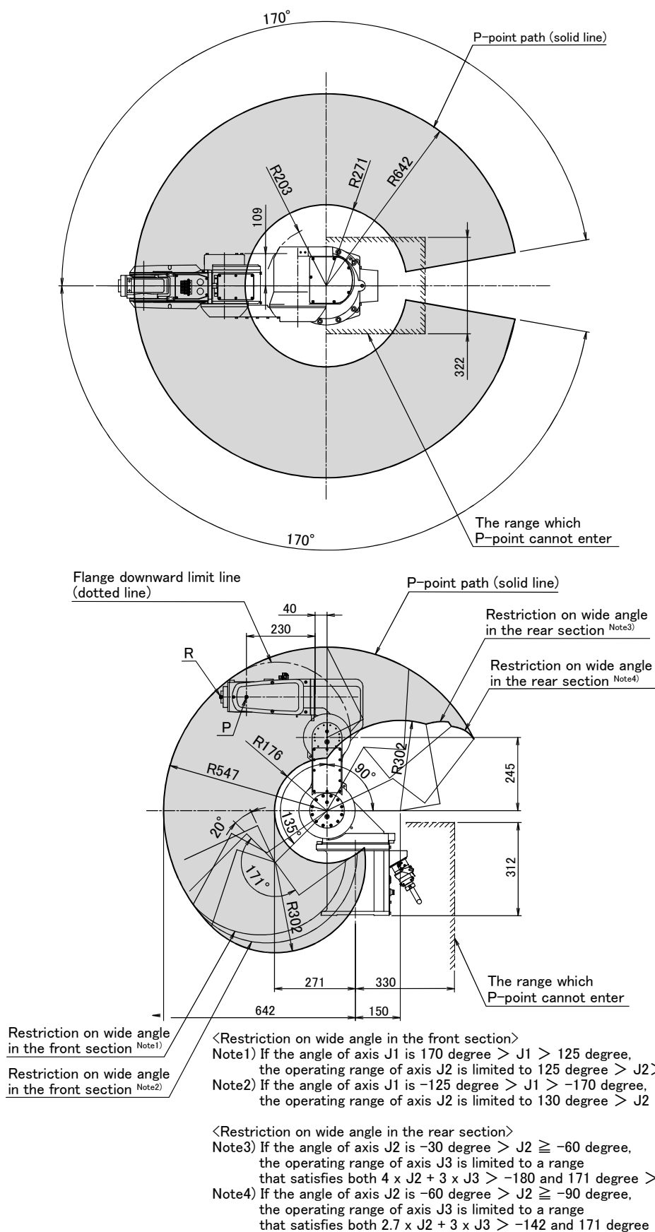
Fig.2-4 : Operating range diagram: (6-axis type)
