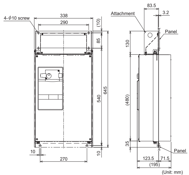
FR-A7CN06
