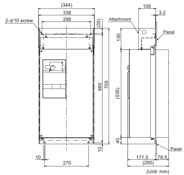
FR-A7CN13
