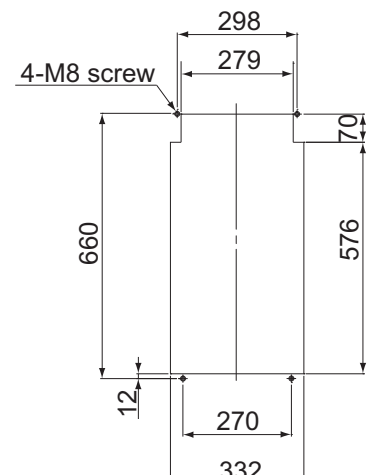
FR-A7CN13
