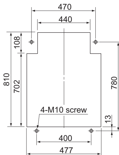
FR-A7CN10
