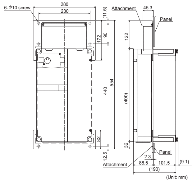
FR-A7CN06
