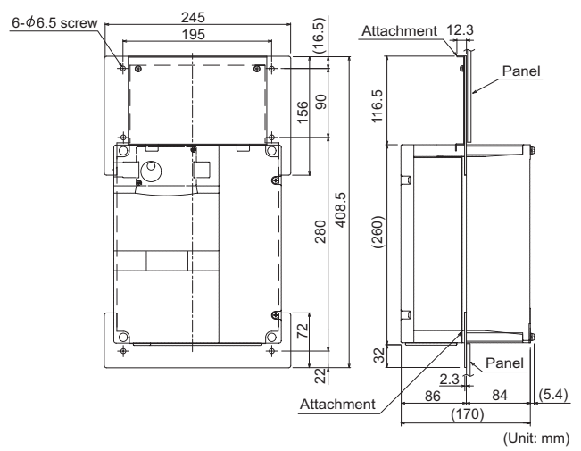
FR-A7CN04
