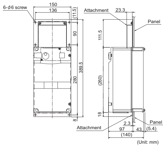
FR-A7CN03
