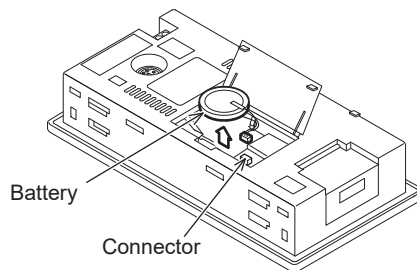
For GT2104-P
