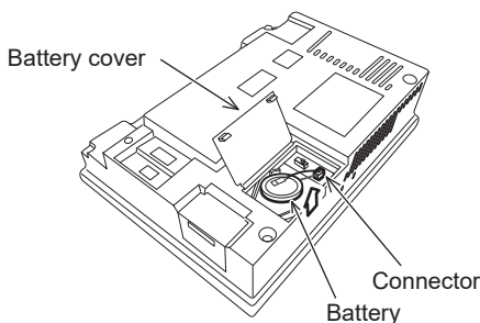
For GT2107-W
