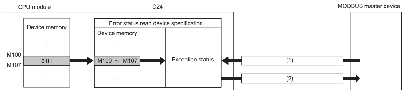
(1) Request message (read exception status (FC: 07))
