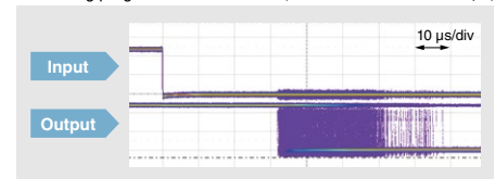
Existing programmable controller (LCPU embedded I/O + interrupts)
