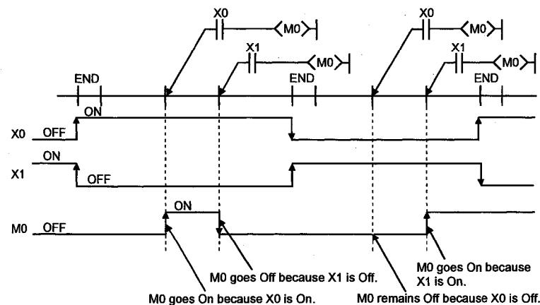
[Timing Chart]
