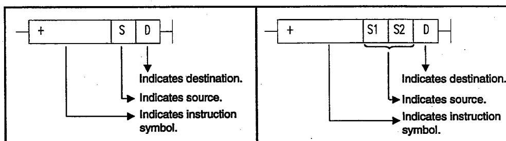
Fig. 2.2 Symbol Representations in Ladder
