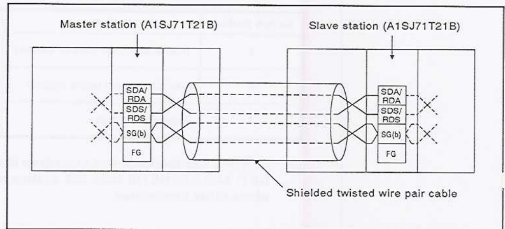
Fig. 4-1 Inter-Station Test
