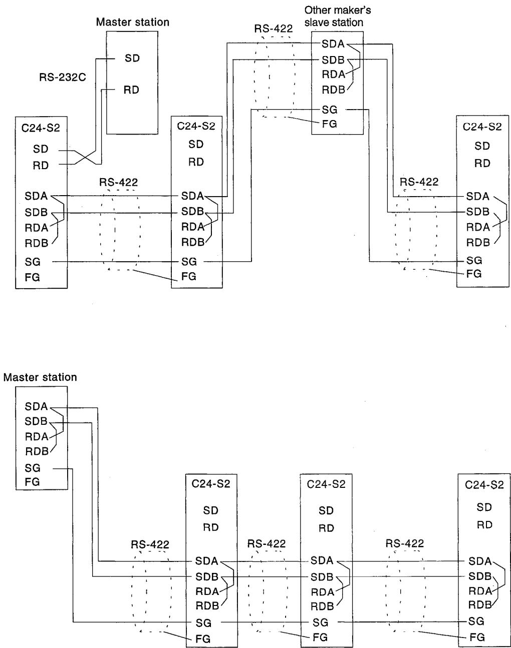
(2-2) Communication through 2 cables
