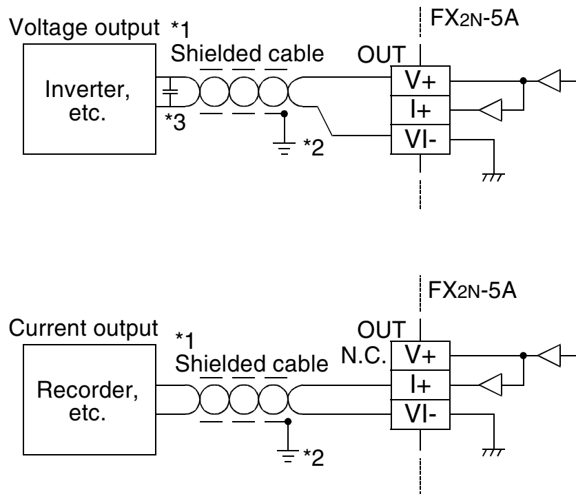
Figure 5.3: Output Wiring
