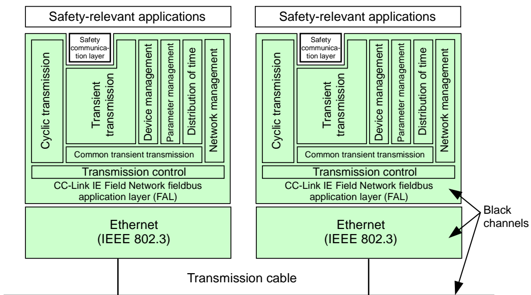
Fig. 2 Protocol layers
