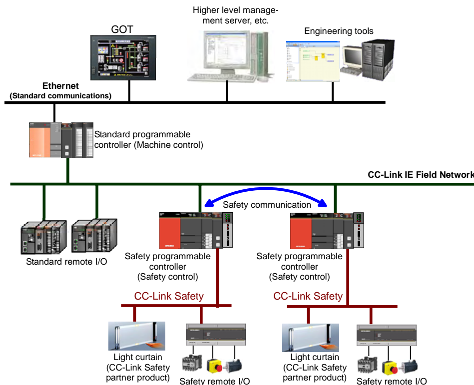
Fig. 1 System configuration
