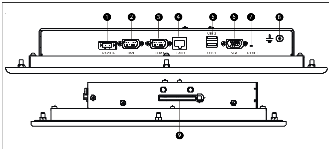
Fig. 3-4: View on interfaces and connectors
