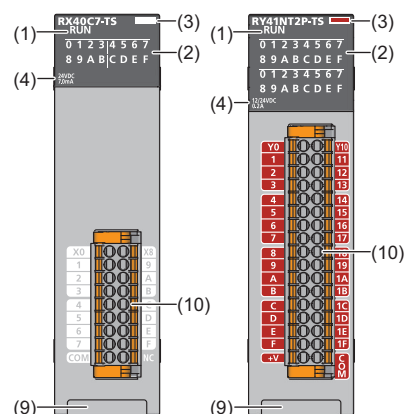
Spring clamp terminal block type
