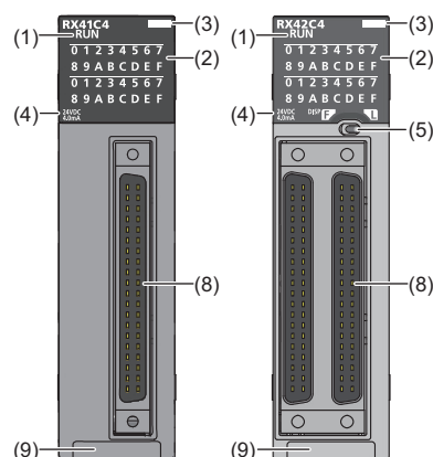
40-pin connector type
