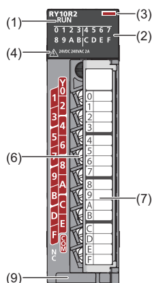
18-point screw terminal block type
