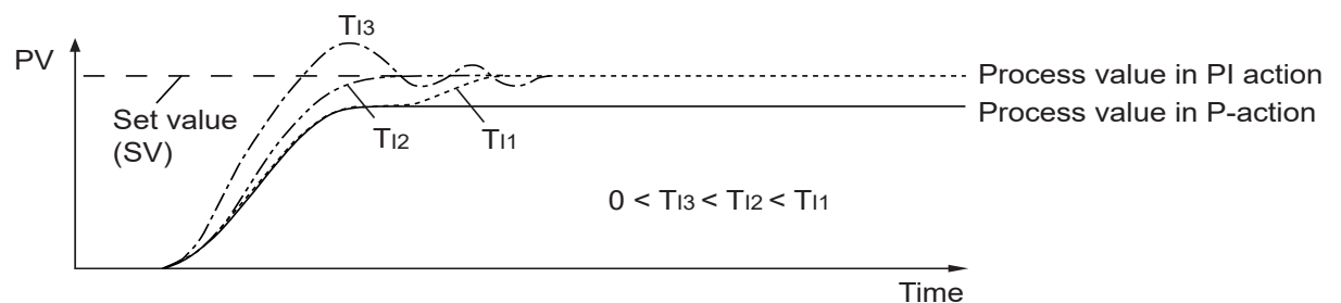
Figure 6.22b. Characteristic response for different T_I parameters
