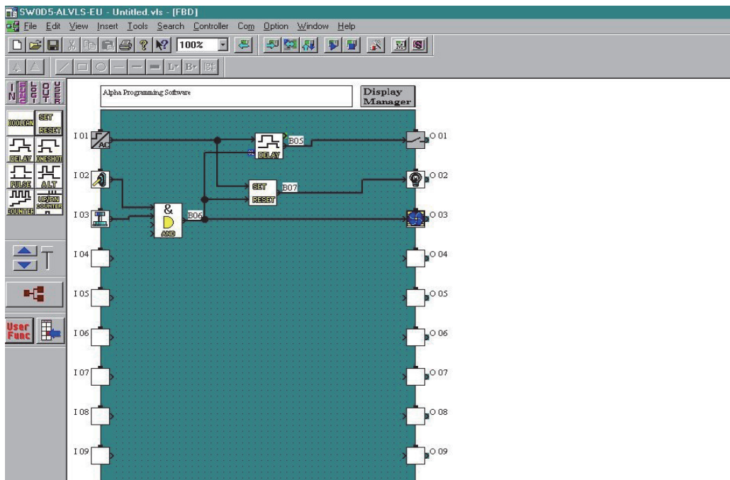
Figure 2.1: AL-PCS/WIN-E Programming Software Ver. 2.50 and upwards
