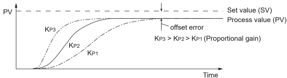
Figure 6.22a. Characteristic response for different K_P parameters
