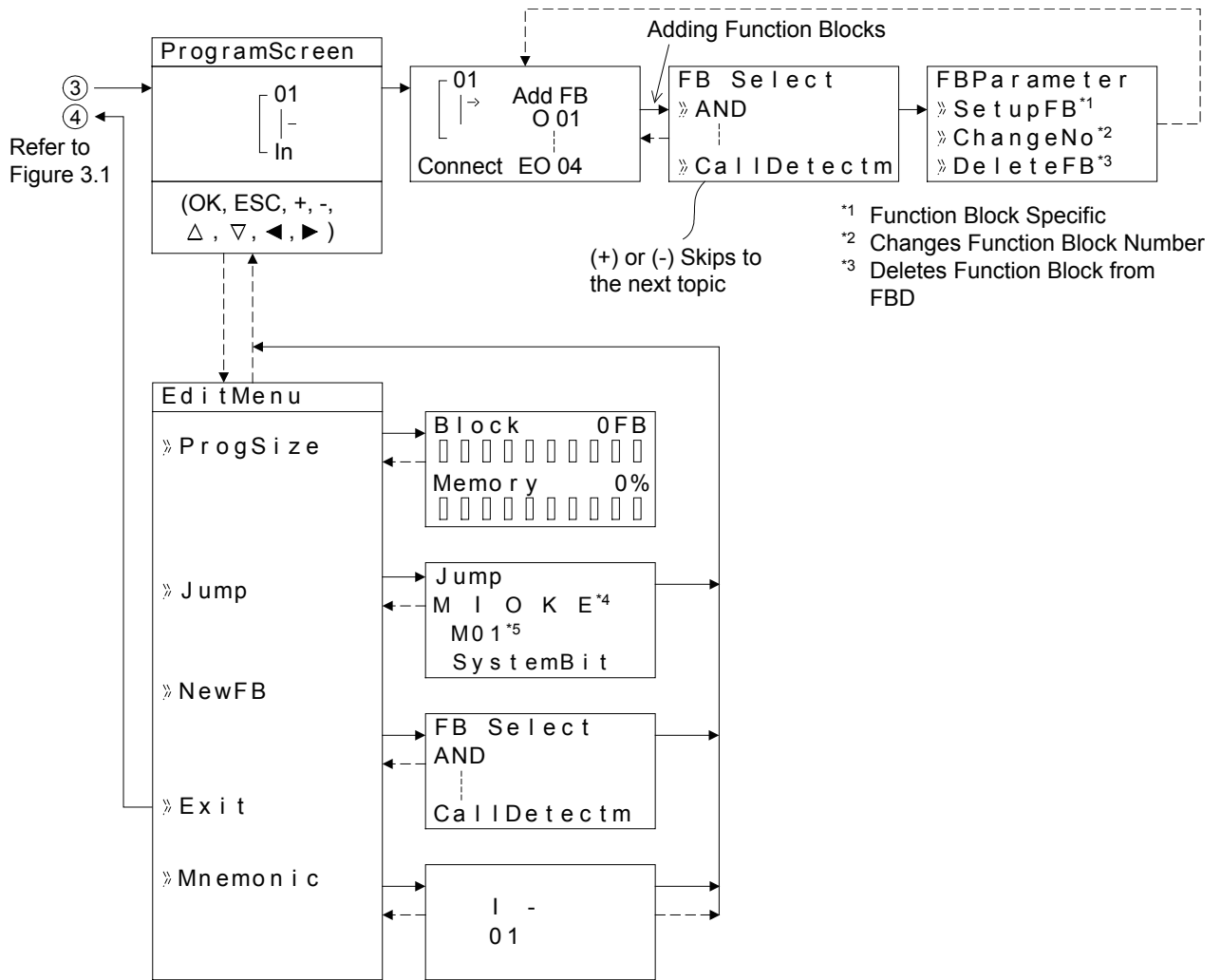
Figure 3.3: ProgEdit Menu in Stop Mode Operation
