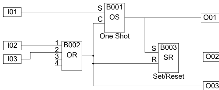
Figure 1.1: Principle of Function Block Programming
