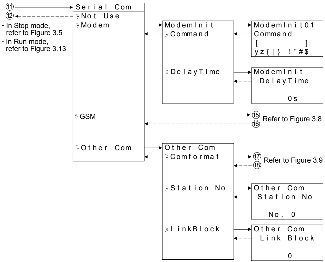
Figure 3.7: Serial Com in Run/Stop Mode Operation (AL2-14MR-*, AL2-24MR-* Only)
