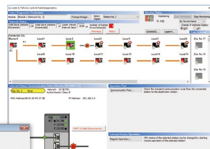
Diagnostics window
