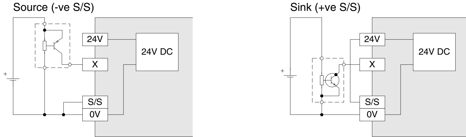
Figure 5.2: Input Circuit Diagrams (Source/Sink)
